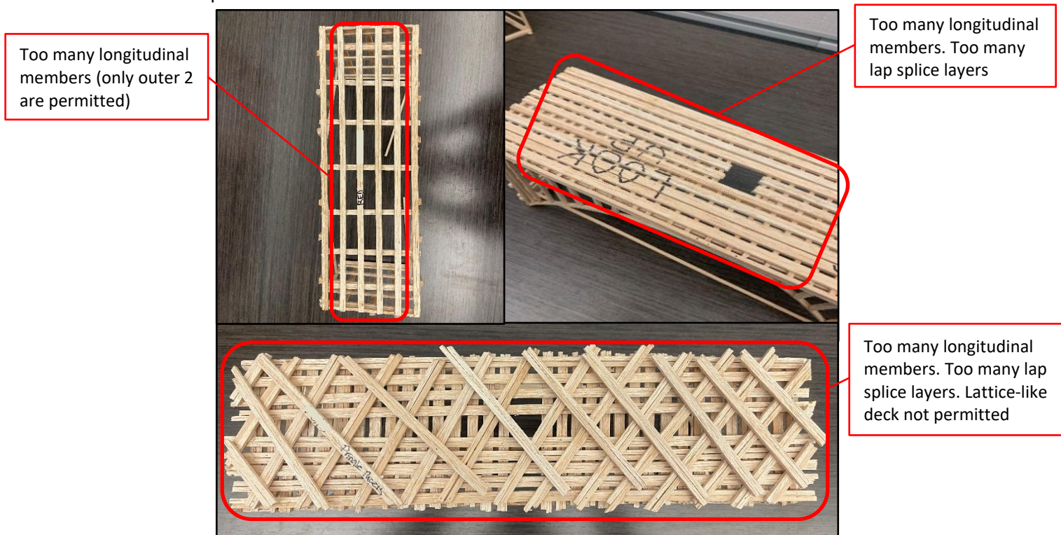
Figure 11. Unacceptable Cross Framing/Deck System
