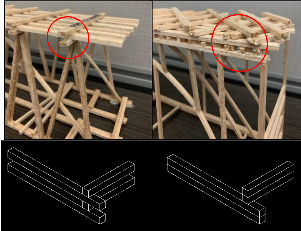
Figure 6. Unacceptable Lamination/Splices
