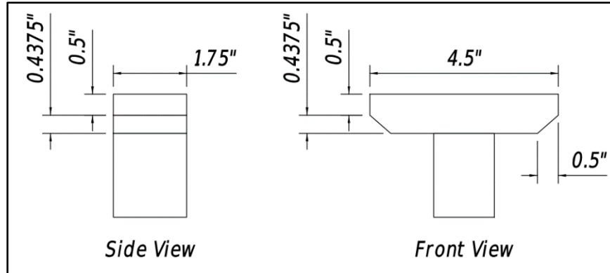
Figure 8. Support Detail
